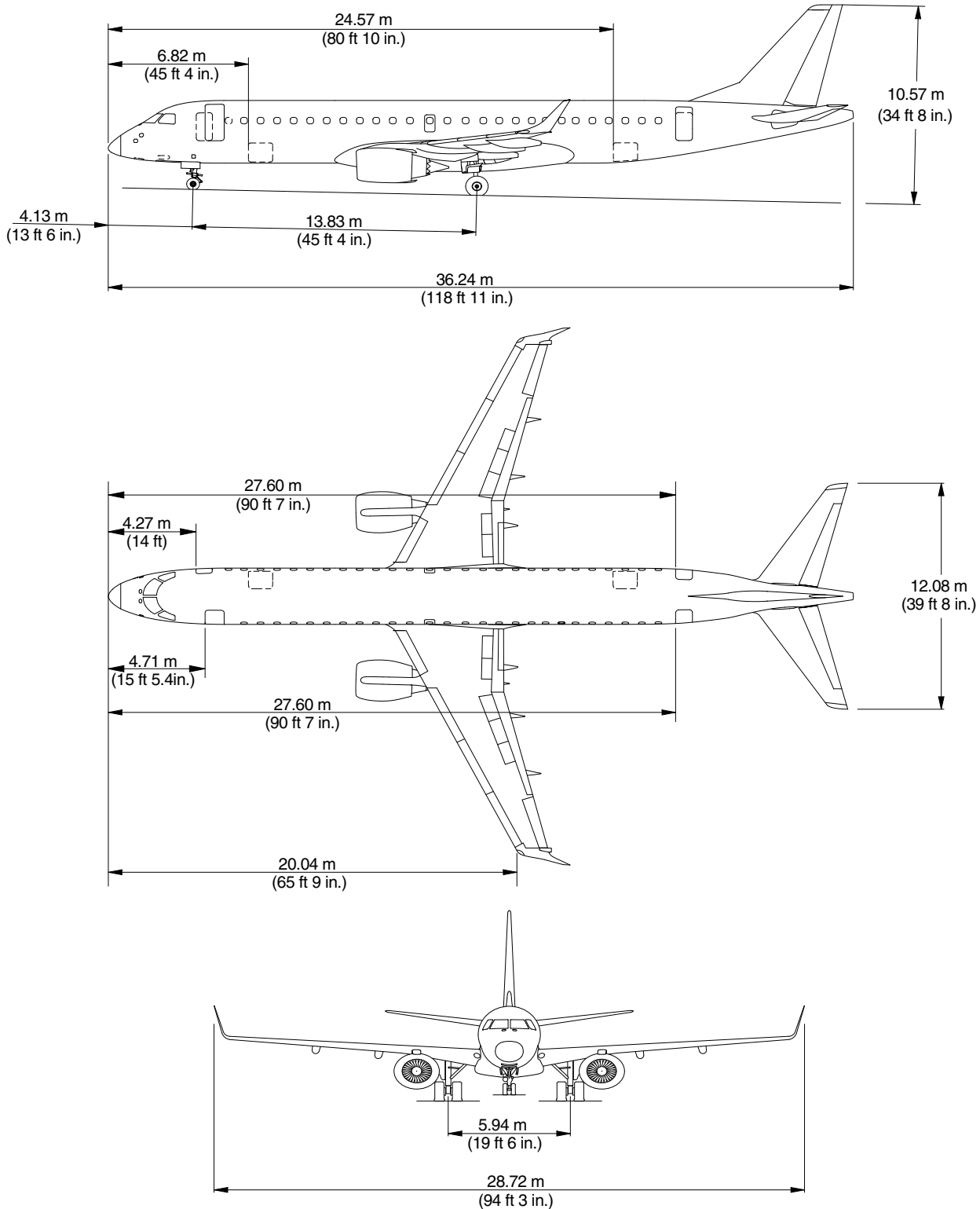
EFFECTIVITY: ALL General Aircraft Dimensions Figure 2.1
