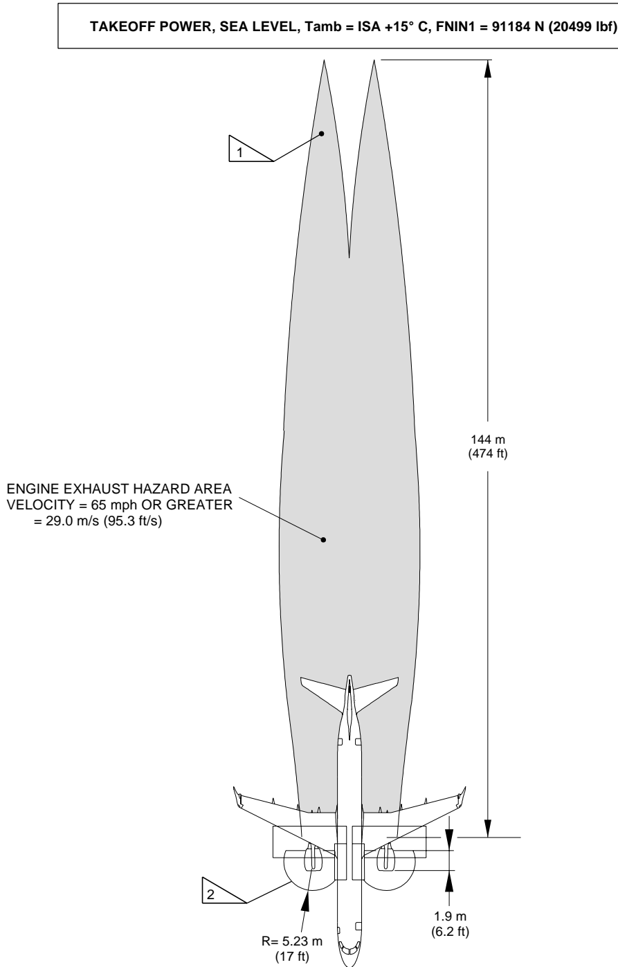
EFFECTIVITY: ALL Hazard Areas - Takeoff Power Figure 6.7
