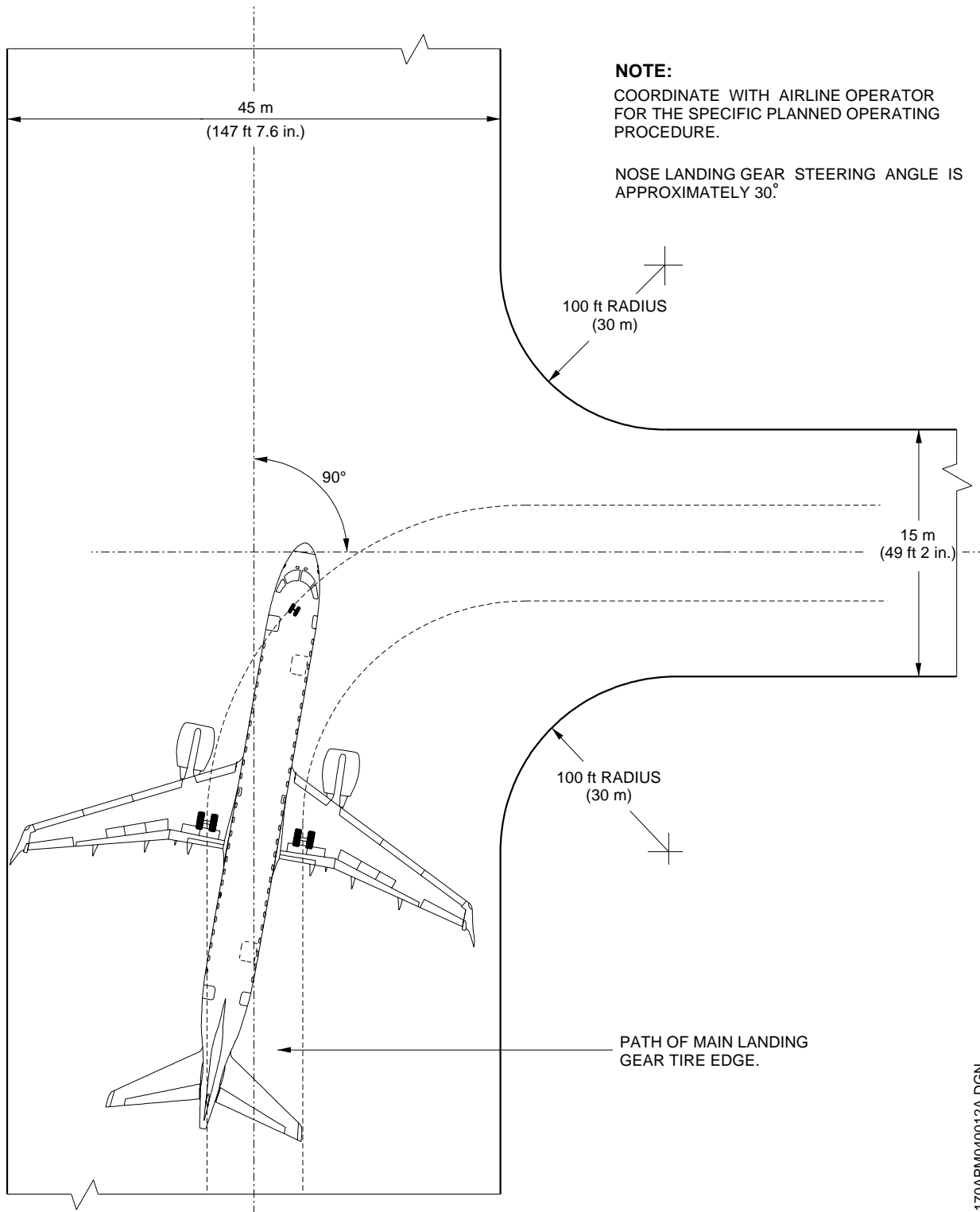
EFFECTIVITY: EMBRAER ACFT 190 LR OR AR MODEL 90° Turn - Runway to Taxiway Figure 4.7
